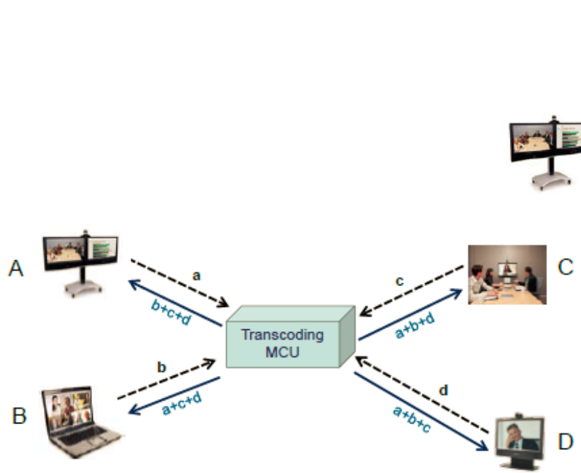
Figure 1: Multipoint call with a transcoding MCU. Note that each endpoint sends and receives ONE stream.
