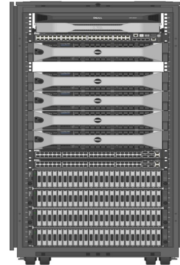
Rack Layout Pre-Integrated Oracle RAC POC
